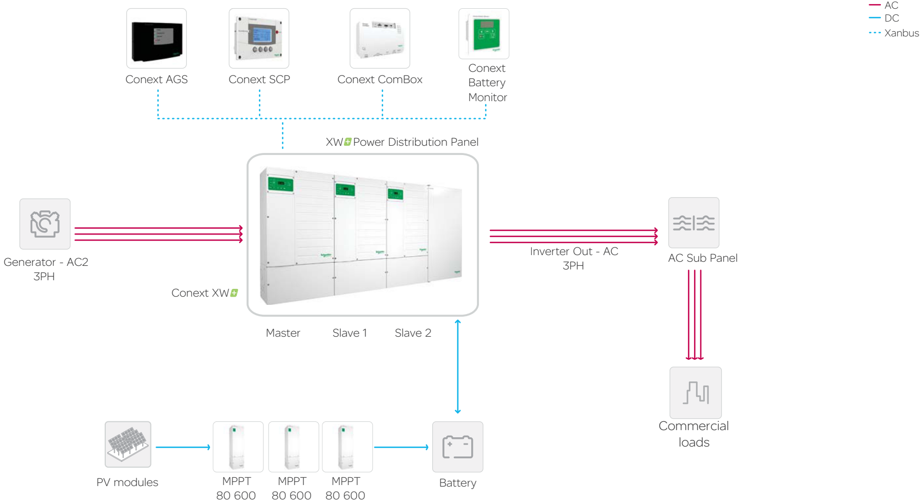
DC Coupled three-phase (230/400VAC) solution with optional AGS/Generator (21.0 or 25.5kW) Three XW+ units are required for three-phase, one per phase.
